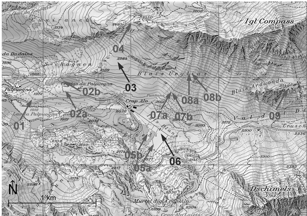
Figure 3. Location of the weather stations within the investigated area. The position of the agrometeorological weather stations (sites 03 and 06) is indicated with a blue arrow, the position of the stations for the near-surface measurements with red arrows. Reproduced by permission of swisstopo (© 2011, JD100042/JA100120).
