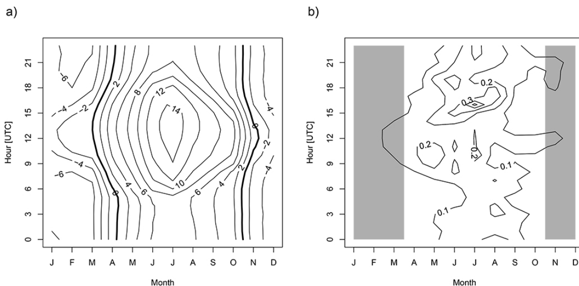
Figure 4. (a) Thermoisopleths diagram (2 °C increments) for the agrometeorological weather station 06 (valley floor) for the period 2006–2008. (b) Same, but for the mean hourly precipitation sum (0.1 mm increments). Gray shaded is the extended winter period where the unheated rain gauge is expected to malfunction.
