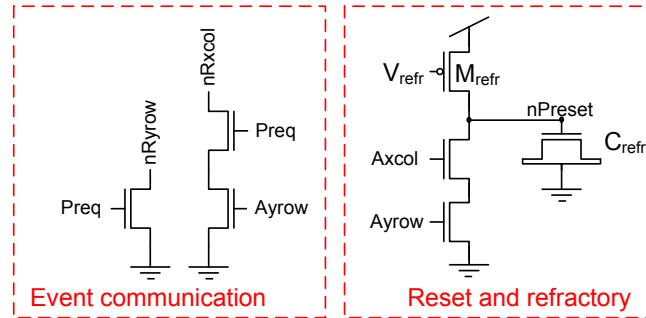
(b) Transistor level circuit of the DVS128.
