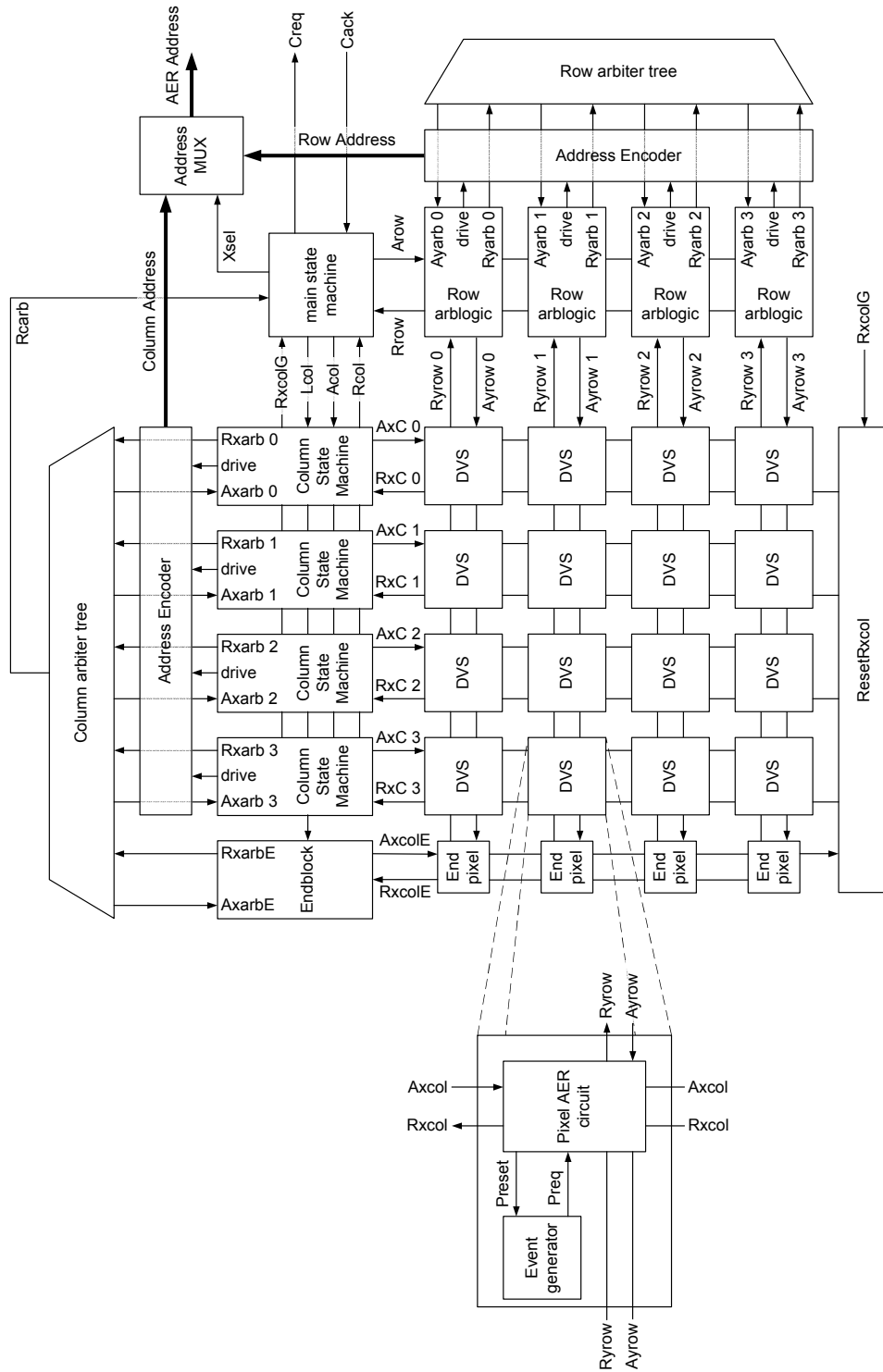
Figure 7.2: Word serial AER block diagram for a 4 × 4 pixel array. The signal names Axcol and Rxcol have been shortened to AxC and RxC .
